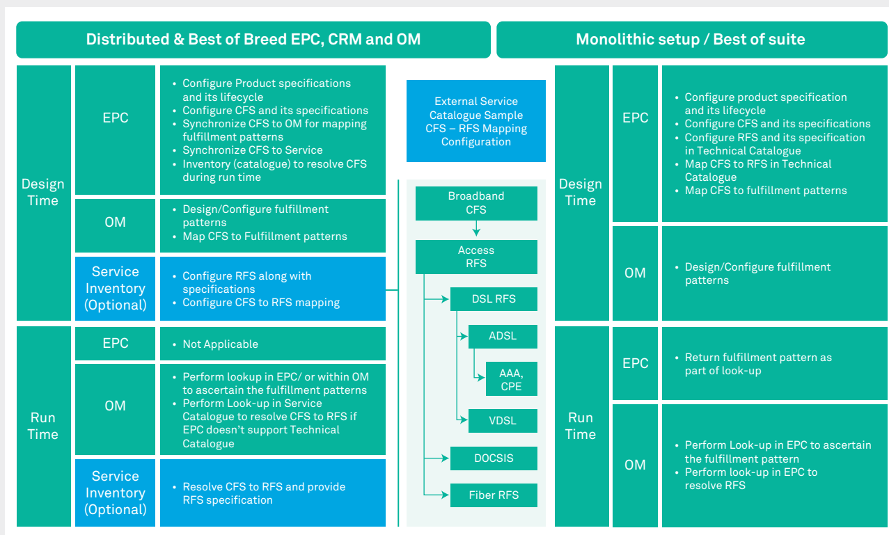
Figure 4: CDOM realization – Best of breed vs Monolithic
