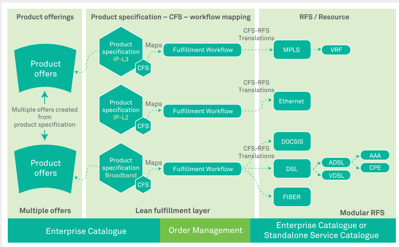
Figure 3: Relationship between PS, CFS, RFS and Resources
