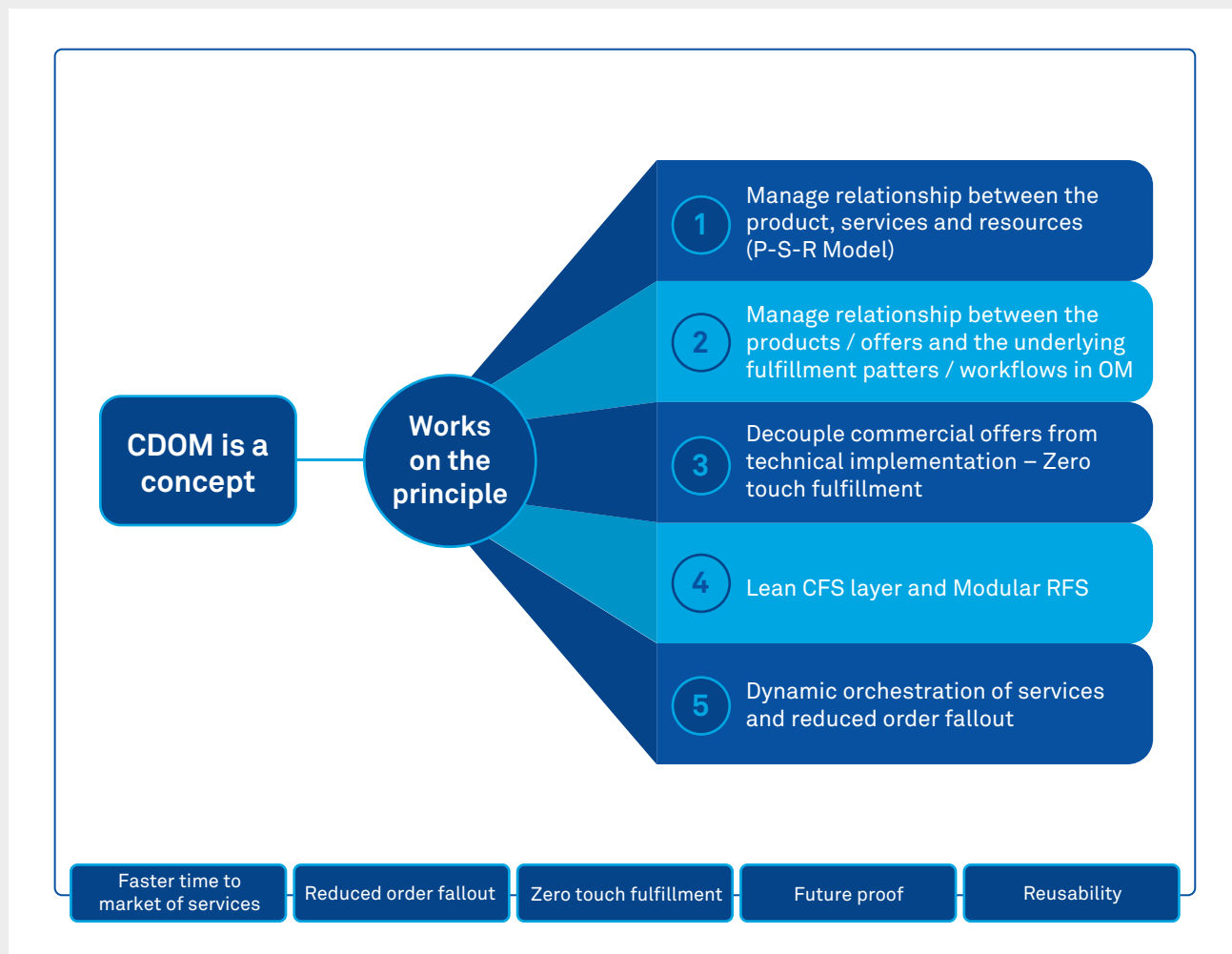
Figure 1: Principles of Catalogue Driven Order Management
